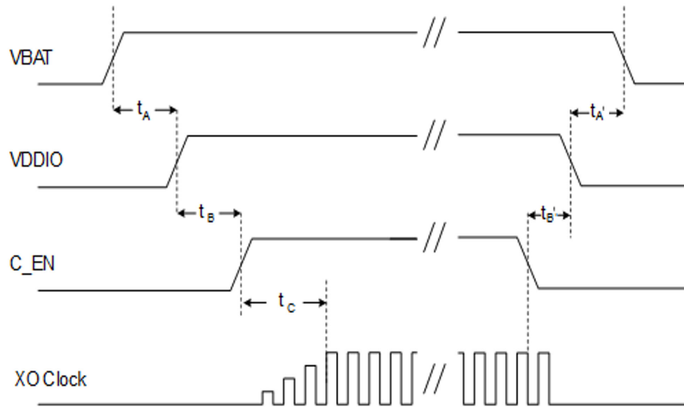
Figure 5-1. Power-up/Power-down Sequence
