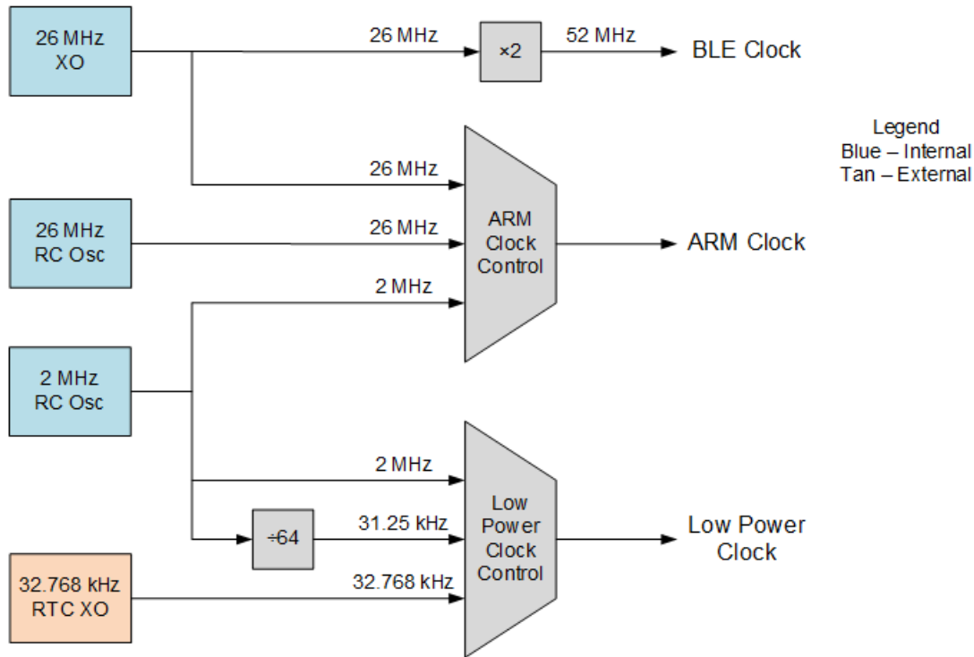
Figure 7-1. Clock Architecture
