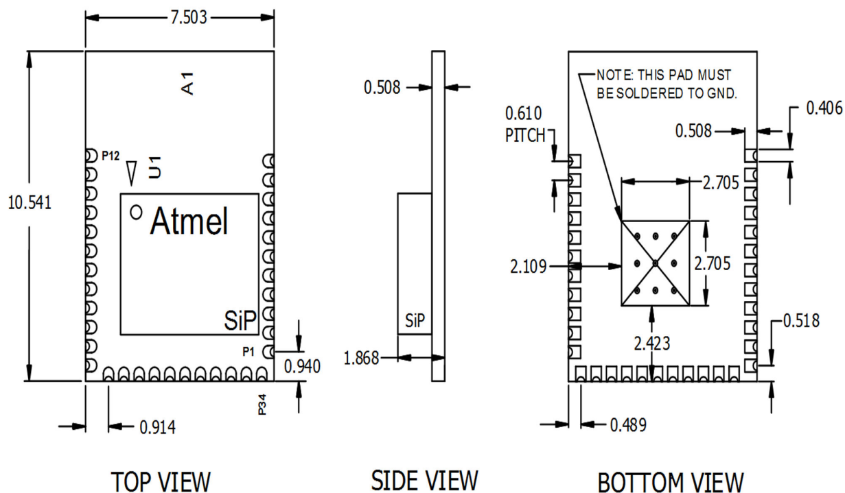
Figure 12-2. ATBTLC1000-ZR110CA Module Package Outline Drawing
